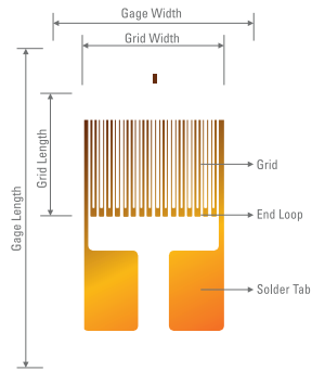
Strain Gauge
